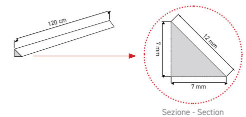
Dettaglio quarter round - Quarter round detail
